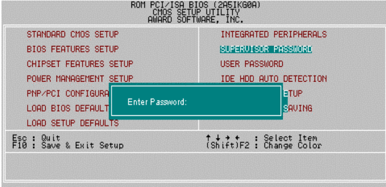
Figure 4.10: Password Setting
