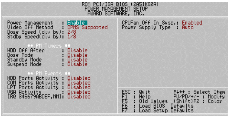
Figure 4.5: Power Management Setup
