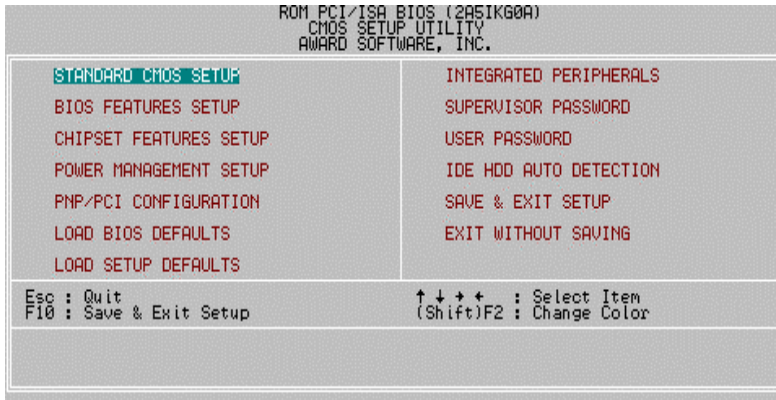
Figure 4.1: Main Menu
