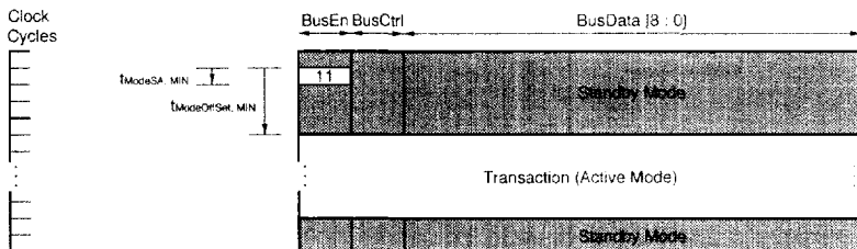
Figure 6-3. ActiveMode/StandbyMode Transition - Early Transaction
