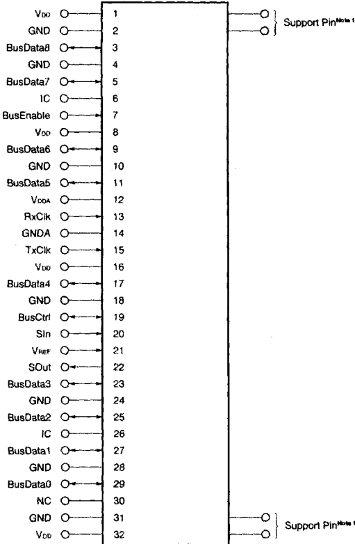
Figure Support Pin Diagram
