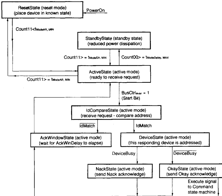
Figure 6-1. Frame State Machine - State Diagram
