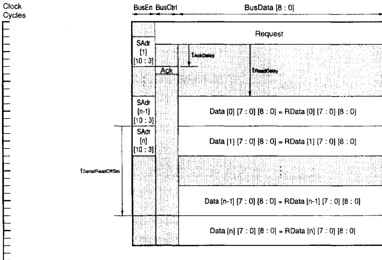
Figure 7-3. Read Transaction with Serial Address Packet
