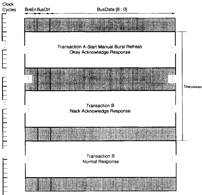
Figure 8-2. Transaction Holdoff Due to Burst Refresh
