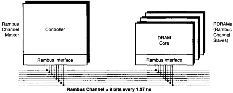
Figure 2-1. Logical Representation
