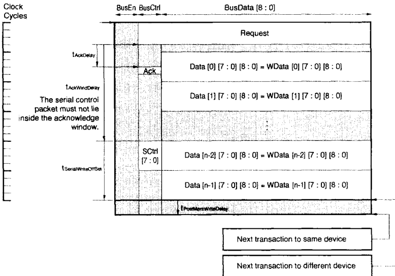
Figure 7-6. Write Transaction with Serial Control Packet
