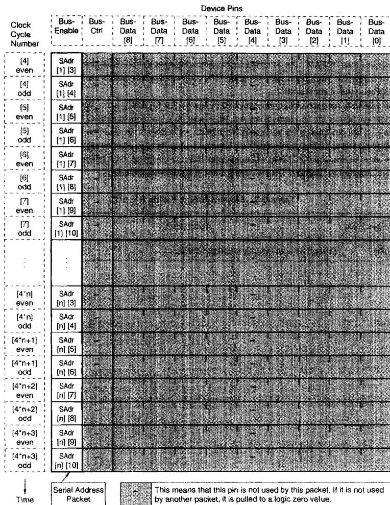
Figure 5-5. Serial Address Packet Format
