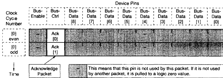
Figure 5-2. Acknowledge Packet Format
