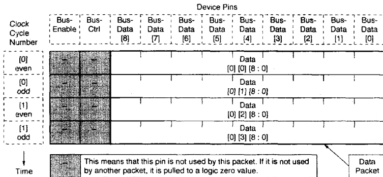
Figure 5-3. Data Packet Format (Register Space)
