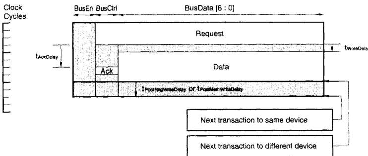
Figure 7-2. Write Transaction
