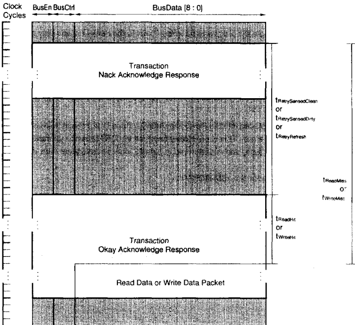
Figure 8-1. Nack Acknowledge Response
