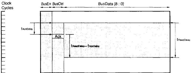
Figure 7-1. Read Transaction
