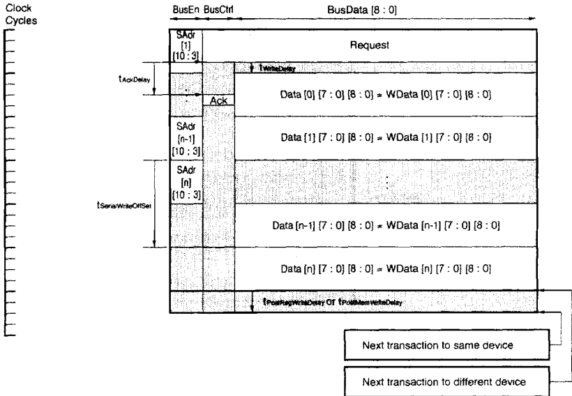
Figure 7-4. Write Transaction with Serial Address Packet
