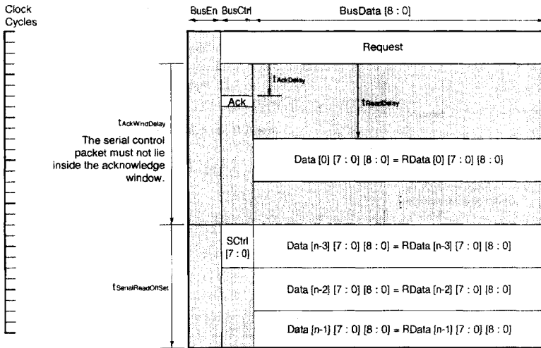
Figure 7-5. Read Transaction with Serial Control Packet
