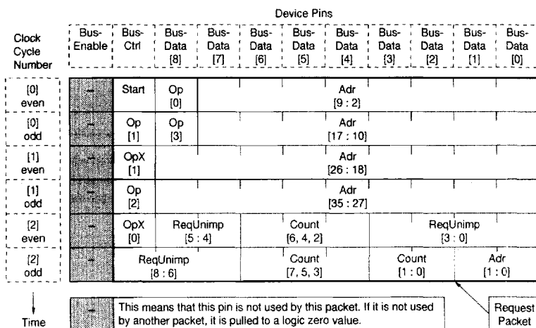
Figure 5-1. Request Packet Format
