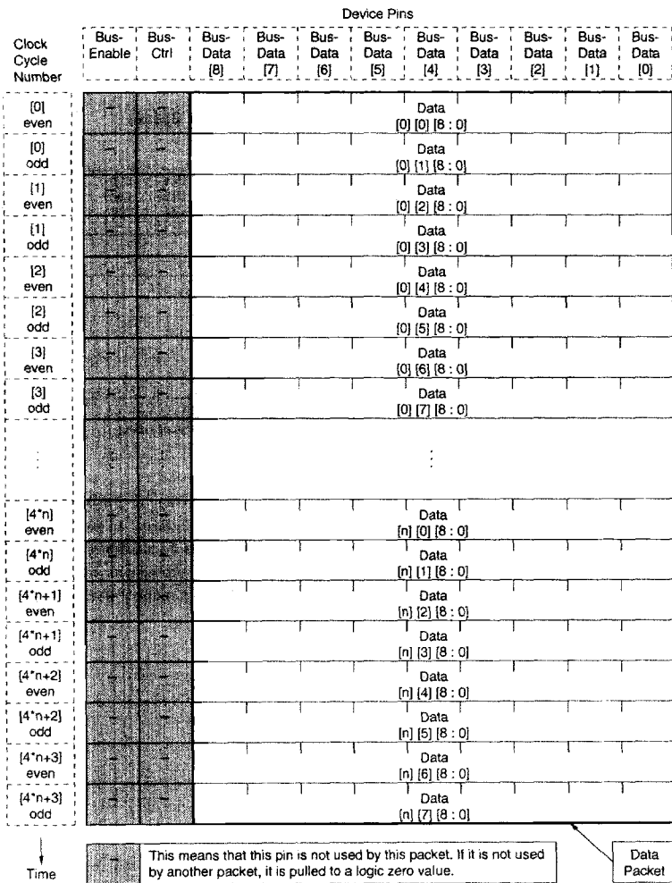
Figure 5-4. Data Packet Format (Memory Space)
