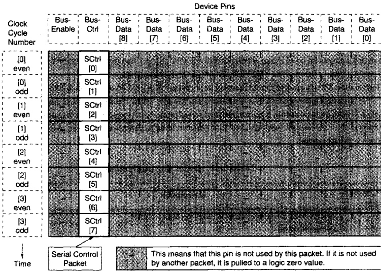
Figure 5-6. Serial Control Packet Format
