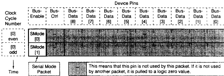
Figure 5-7. Serial Mode Packet Format
