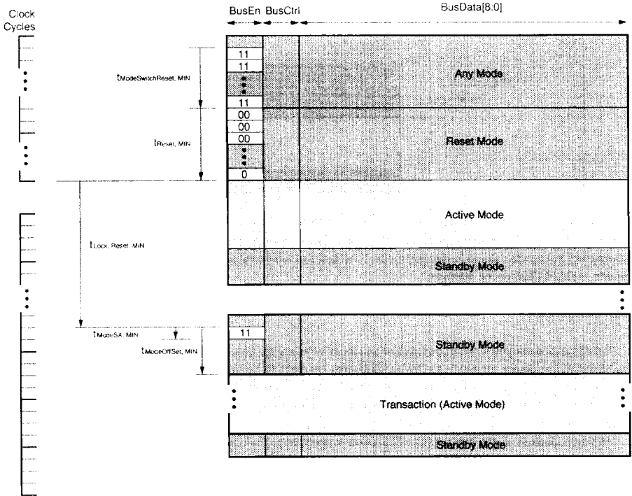
Figure 6-4. ResetMode to ActiveMode Transition
