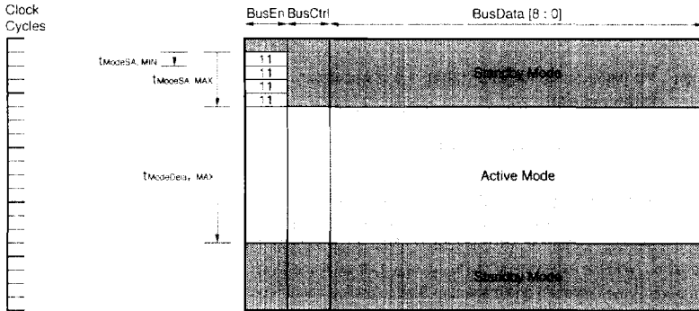
Figure 6-2. Basic ActiveMode/StandbyMode Transitions
