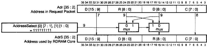
Figure 9-1. AddressMapping Hardware
