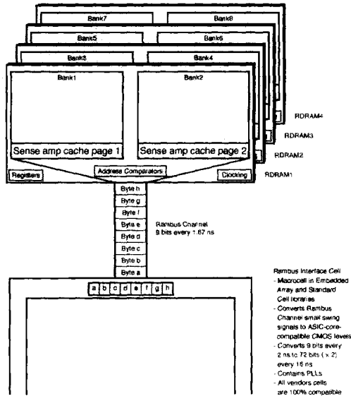
Figure 3-1. Converting the Channel Data Rate
